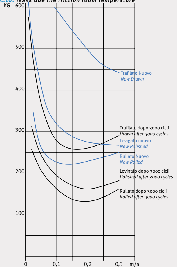
Pic.10: leaks due the friction room temperature
