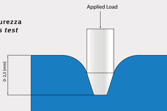
Durometer hardness test
